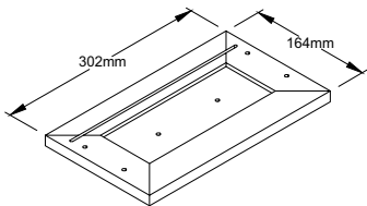
DRAWER FRONT Qty:1
