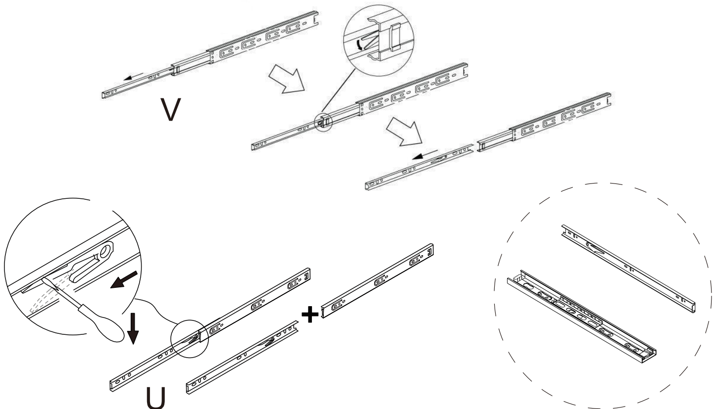
Hardware disassembly example
