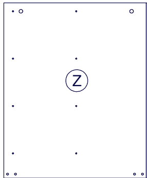
710x580x16mm
