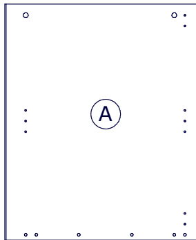
710x580x16mm
