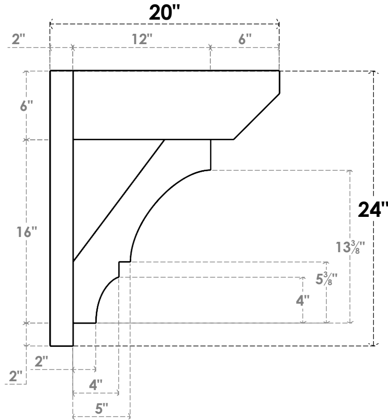
SIDE PROFILE
