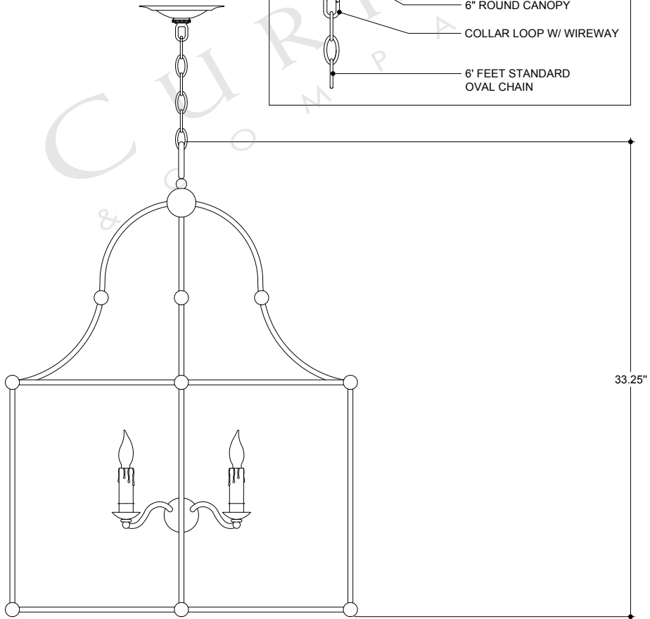
FRONT VIEW
