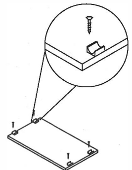
4. Place the cross screws into the buckle and tighten with a screwdriver.
