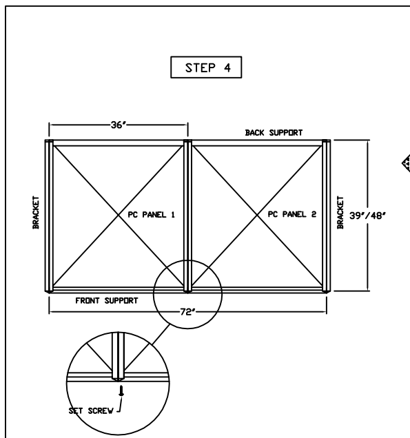
DOOR AND WINDOW AWNING 2 PANELS - SOLID
