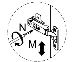
1. VERTICAL ADJUSTMENT VIA SLOT IN THE MOUNTING PLATE
