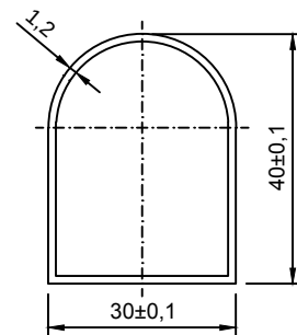
PROFILE DETAIL
