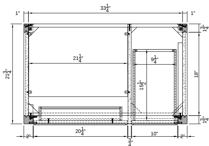
TOP VIEW OF VANITY CABINET
