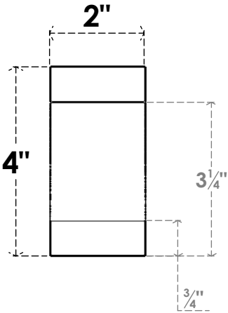
FRONT PROFILE
