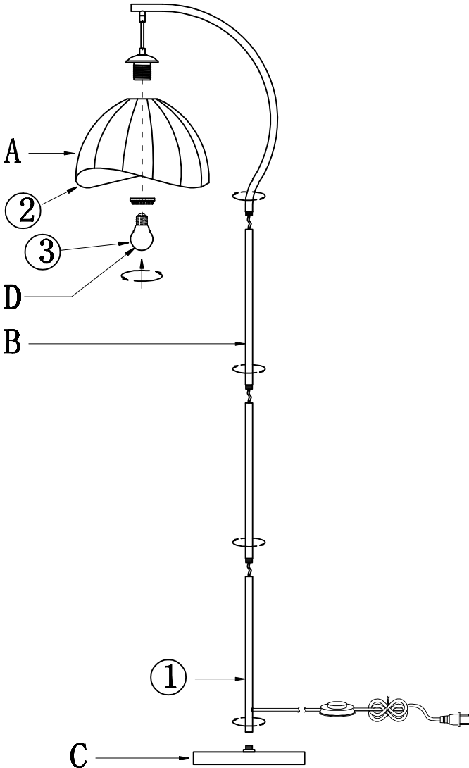
Installation sequence diagram
