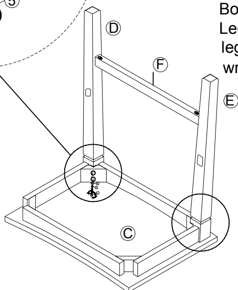
DETAIL A
