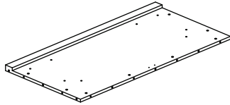
2 (1000*500*30mm x1)
