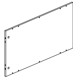
8 (720*380*12mm x2)
