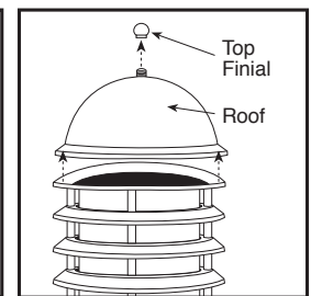
Figure 6 Louver Fixtures
