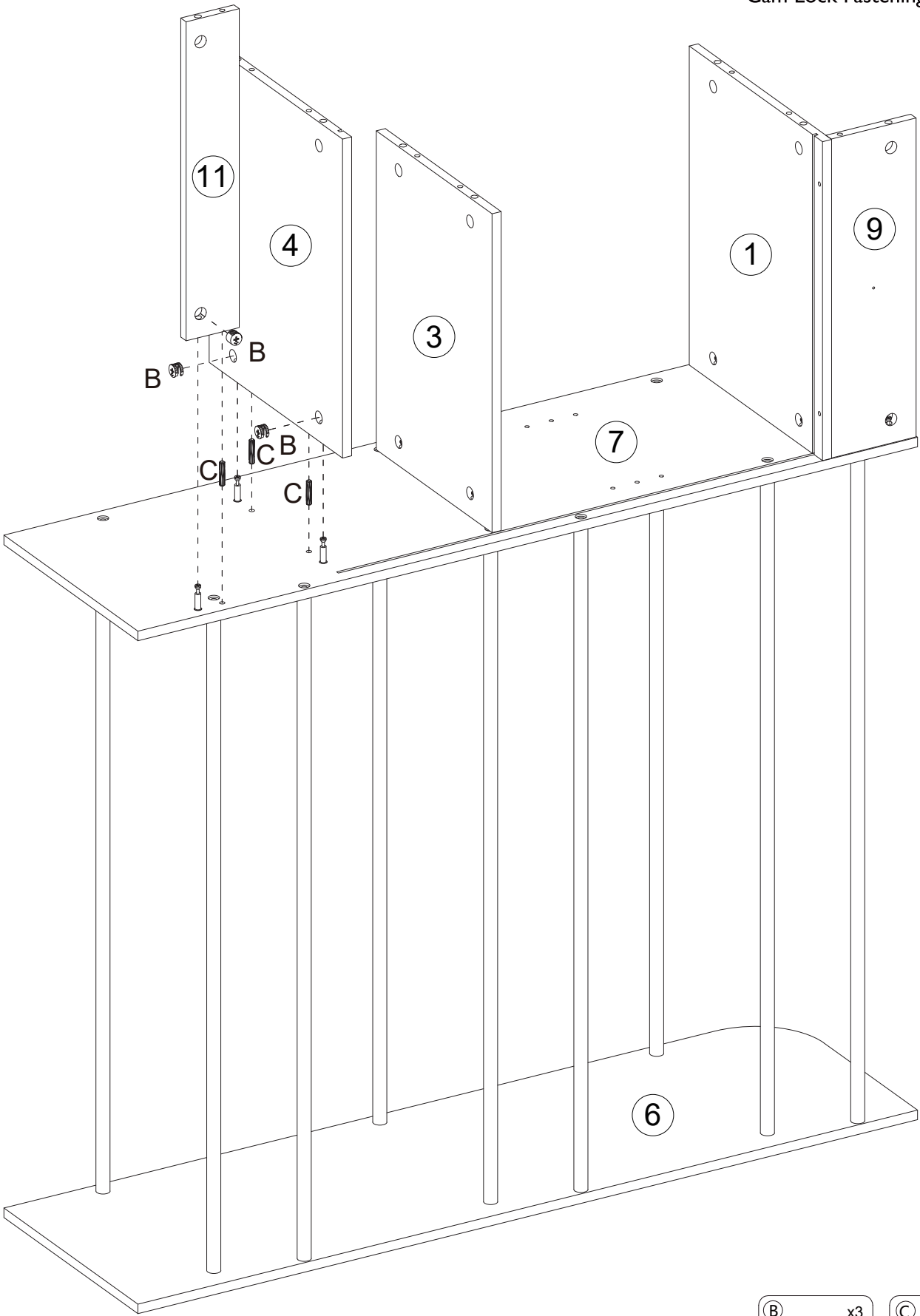
Cam Lock Fastening System
