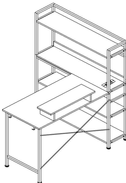
Shelf on Left installation (P1~3,P5~6)
