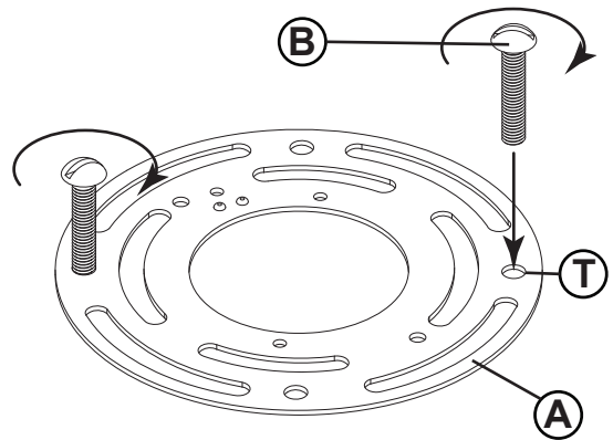
DRAWING 2 - MOUNTING
