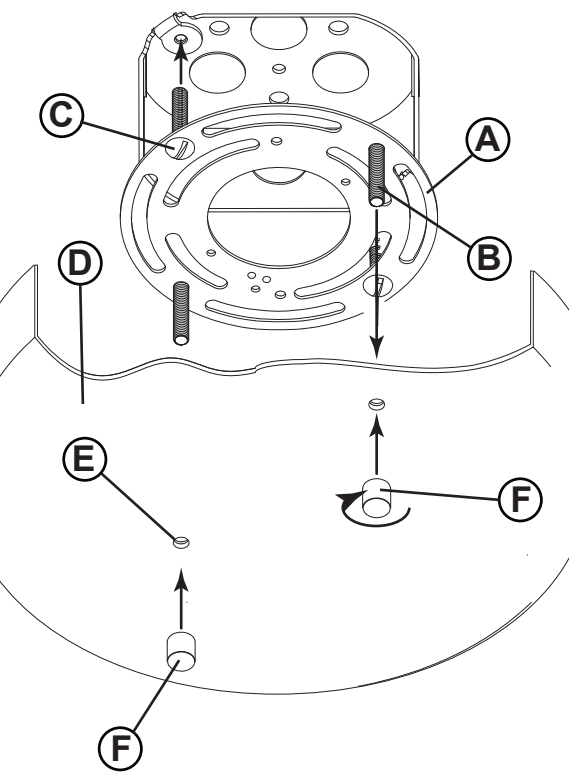
DRAWING 2 - MOUNTING
