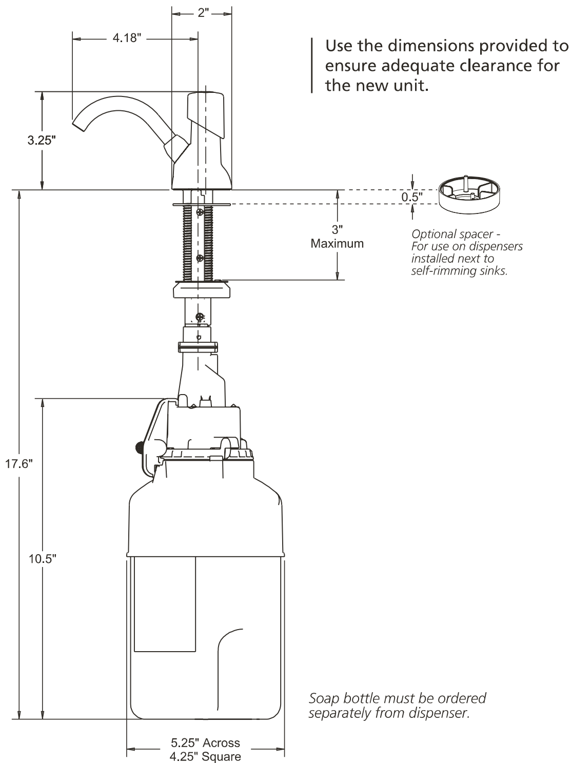
Side View
