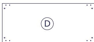
● BA1522 800x356x38mm
