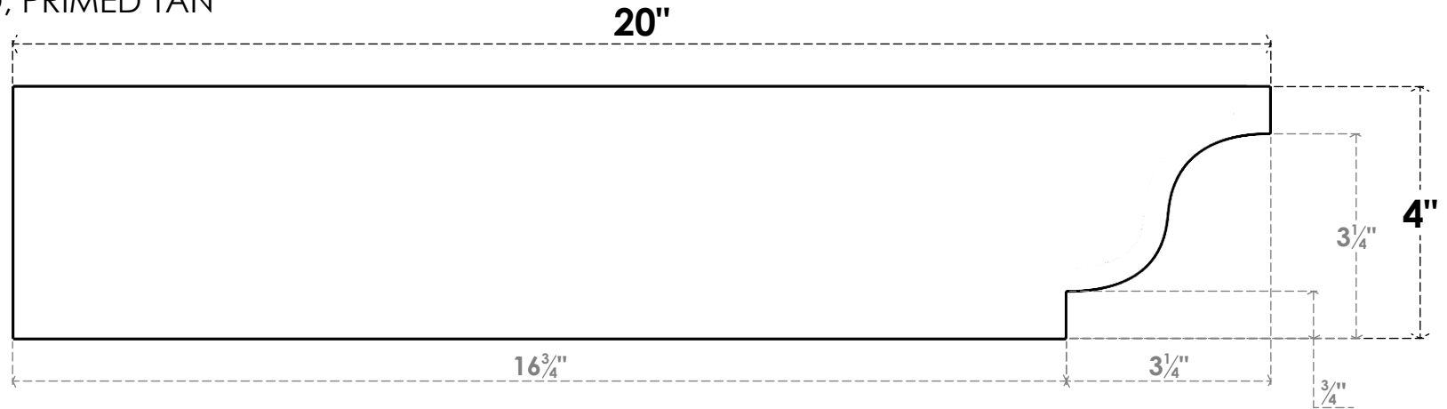
SIDE PROFILE
