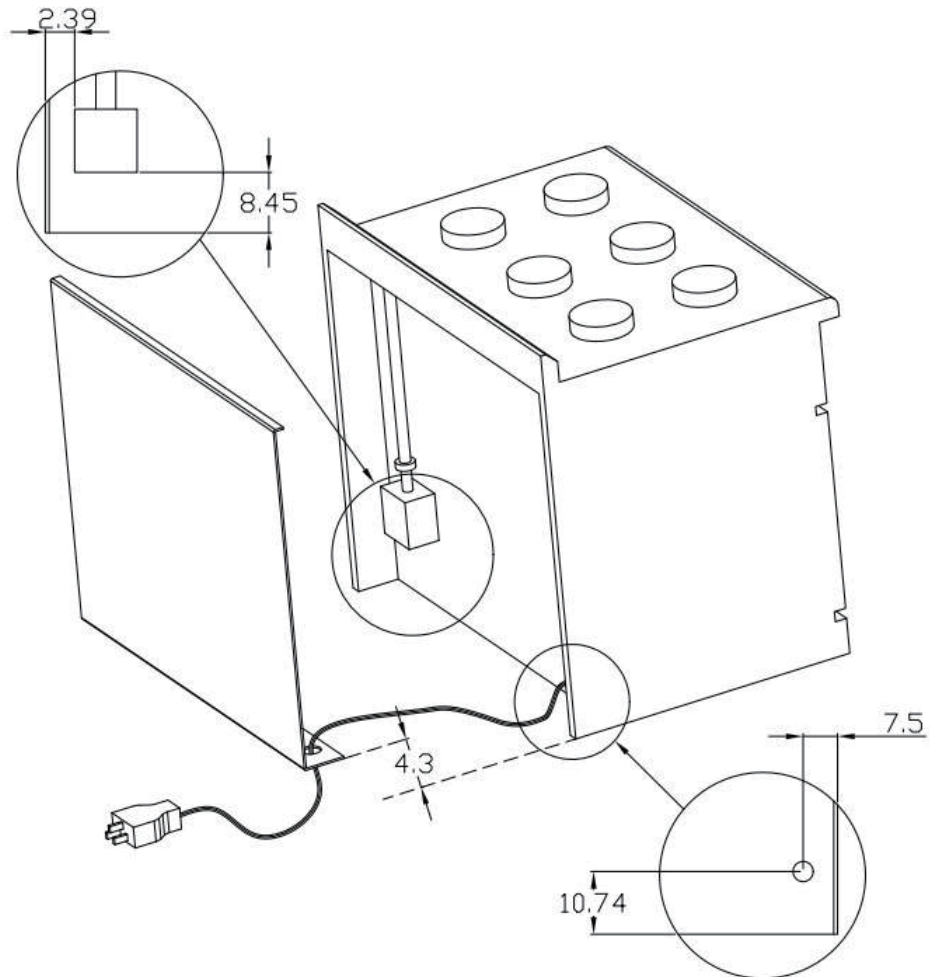
Installation for KOS-RG 30 and 36 inches Gas Range
