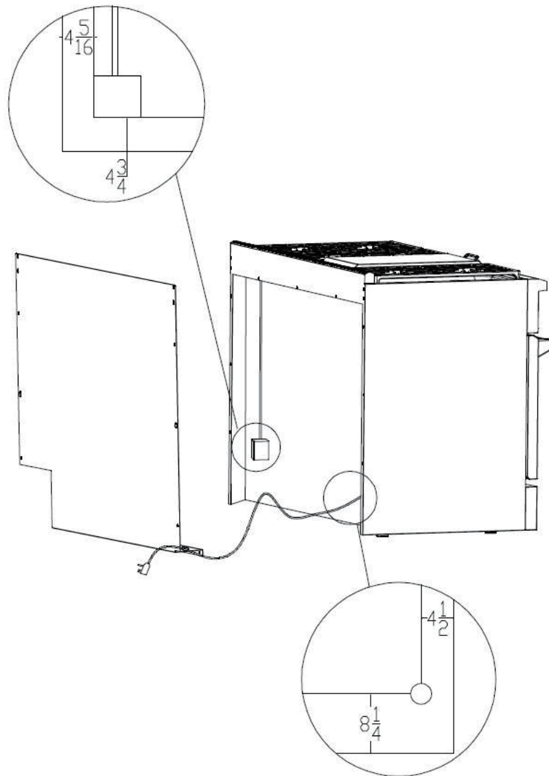
Back Layout for KOS-RG 40 inches Gas Range
