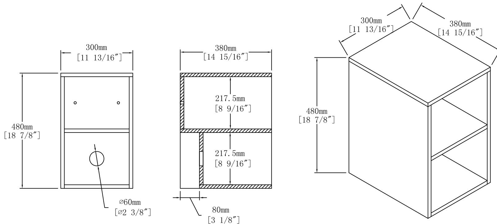
Front View
