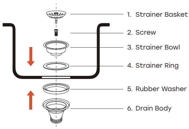
Basket Strainer Assembly Installation
