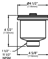
Model #: BST-1 Dimensions: \varnothing 4\ 1/2" x 4 1/2"
