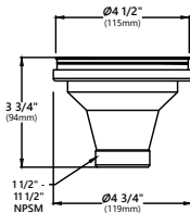
Model #: ST-2 Dimensions: \varnothing 4\ 1/2" x 3 3/4"
