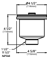
Model #: BST-2 Dimensions: \varnothing 4\ 1/2" x 4 1/2"
