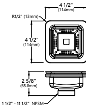
Model #: ST-3 Dimensions: 4 1/2" x 4 1/2" x 2 5/8"
