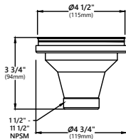
Model #: ST-1 Dimensions: \varnothing 4\ 1/2" x 3 3/4"
