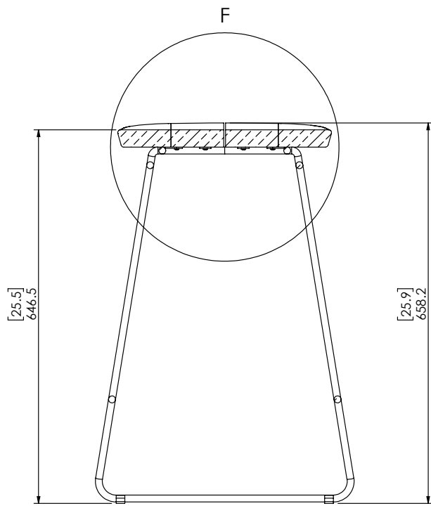
SECTION VIEW
