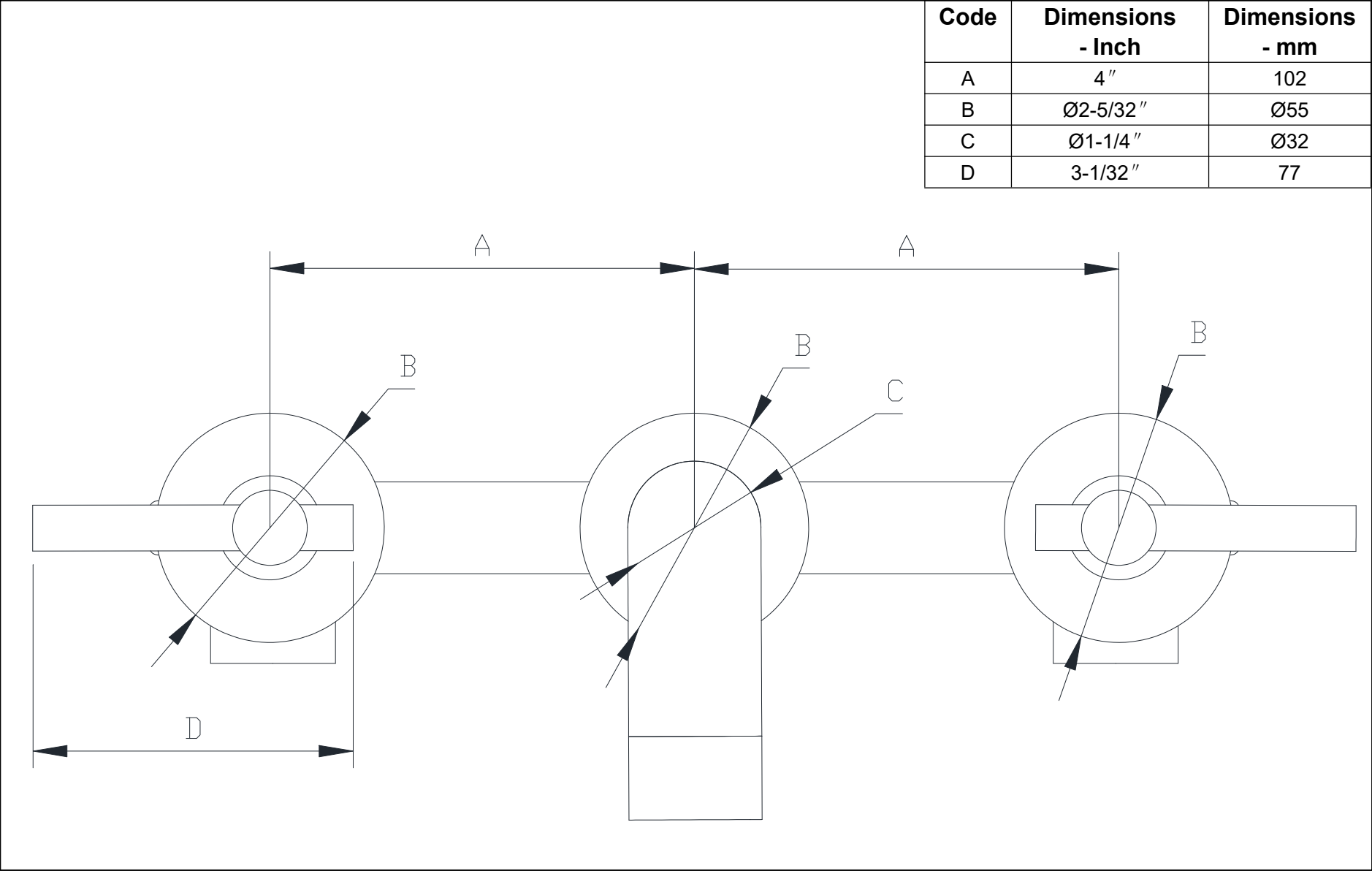
FRONT VIEW
