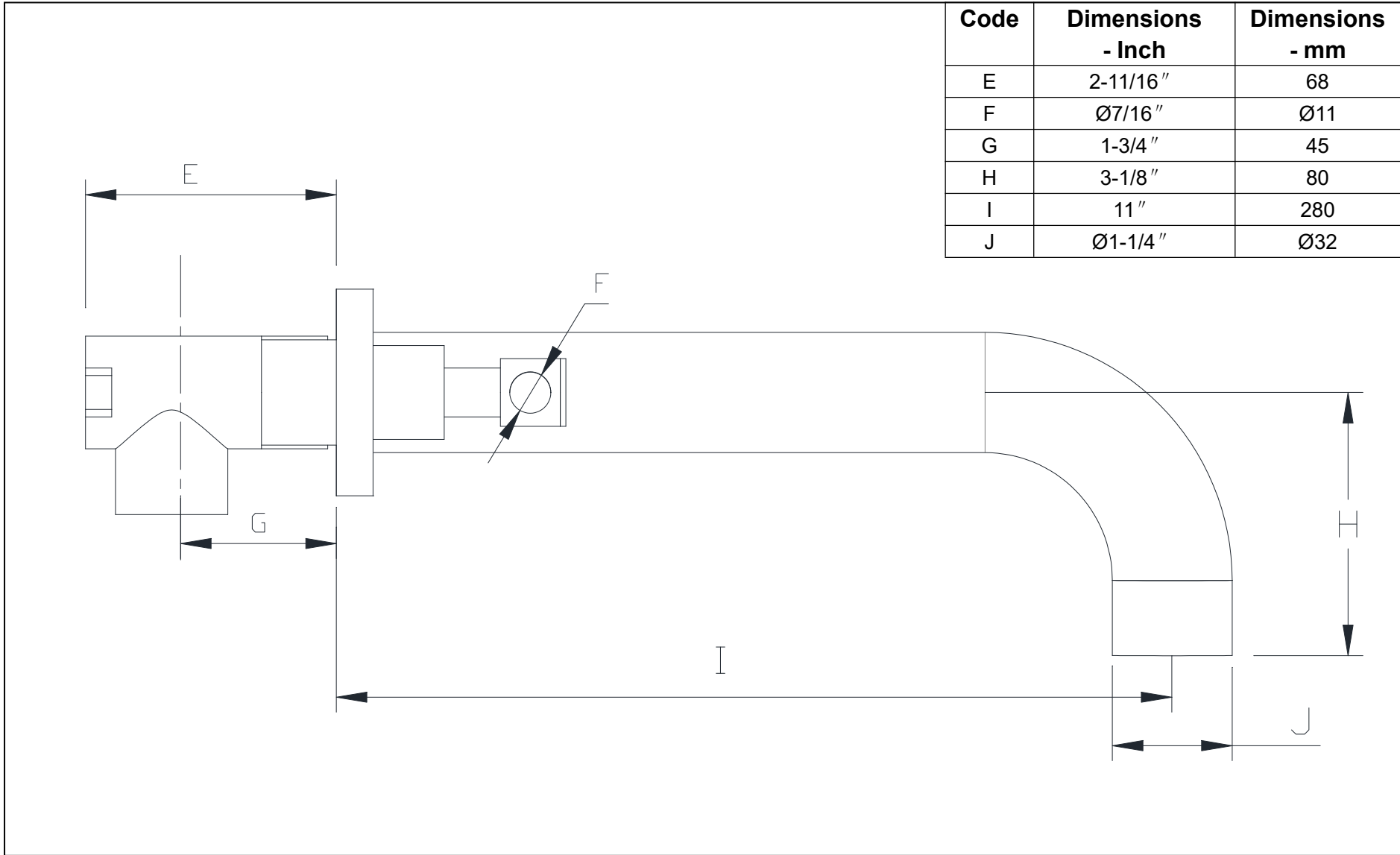
SIDE VIEW
