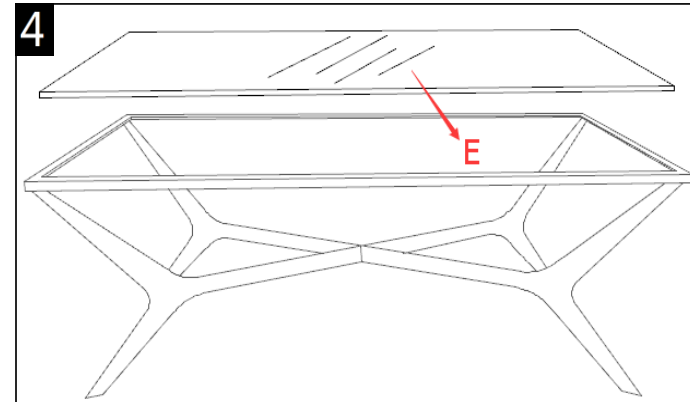
Step 4 Carefully place the Top glass( E) .
