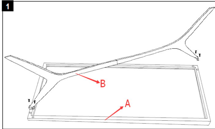
Step 1 Assemble the Leg(B) Top shelf(A) together using 4 screws(D).
