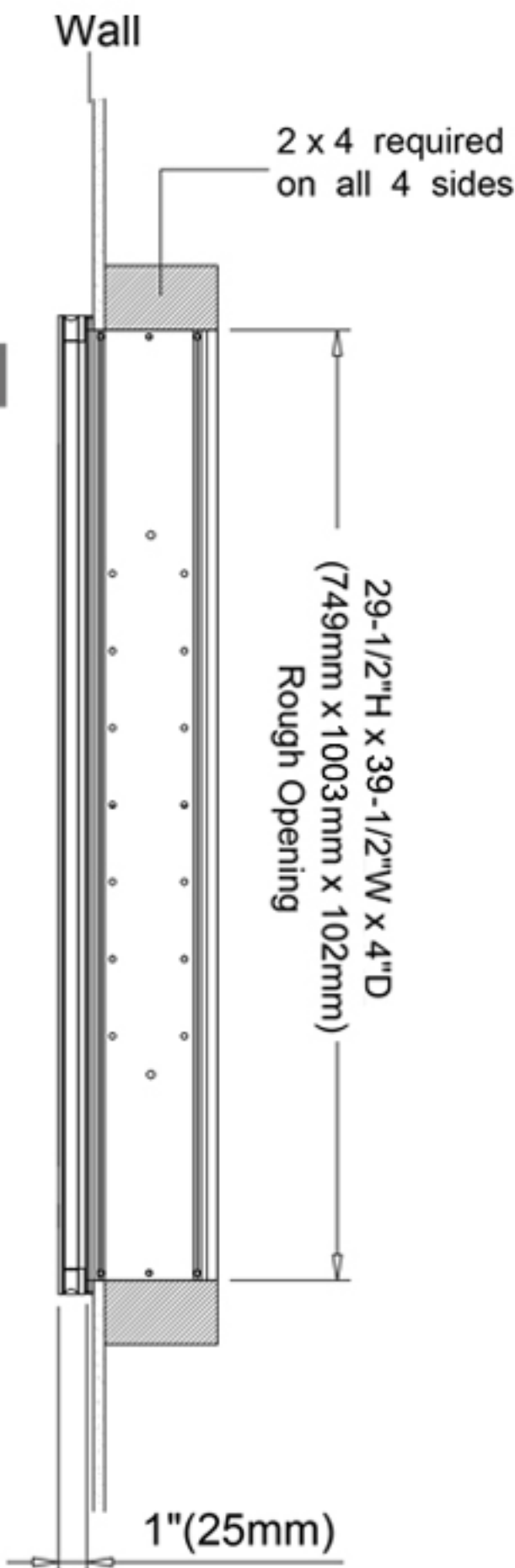
Recessed Mount
