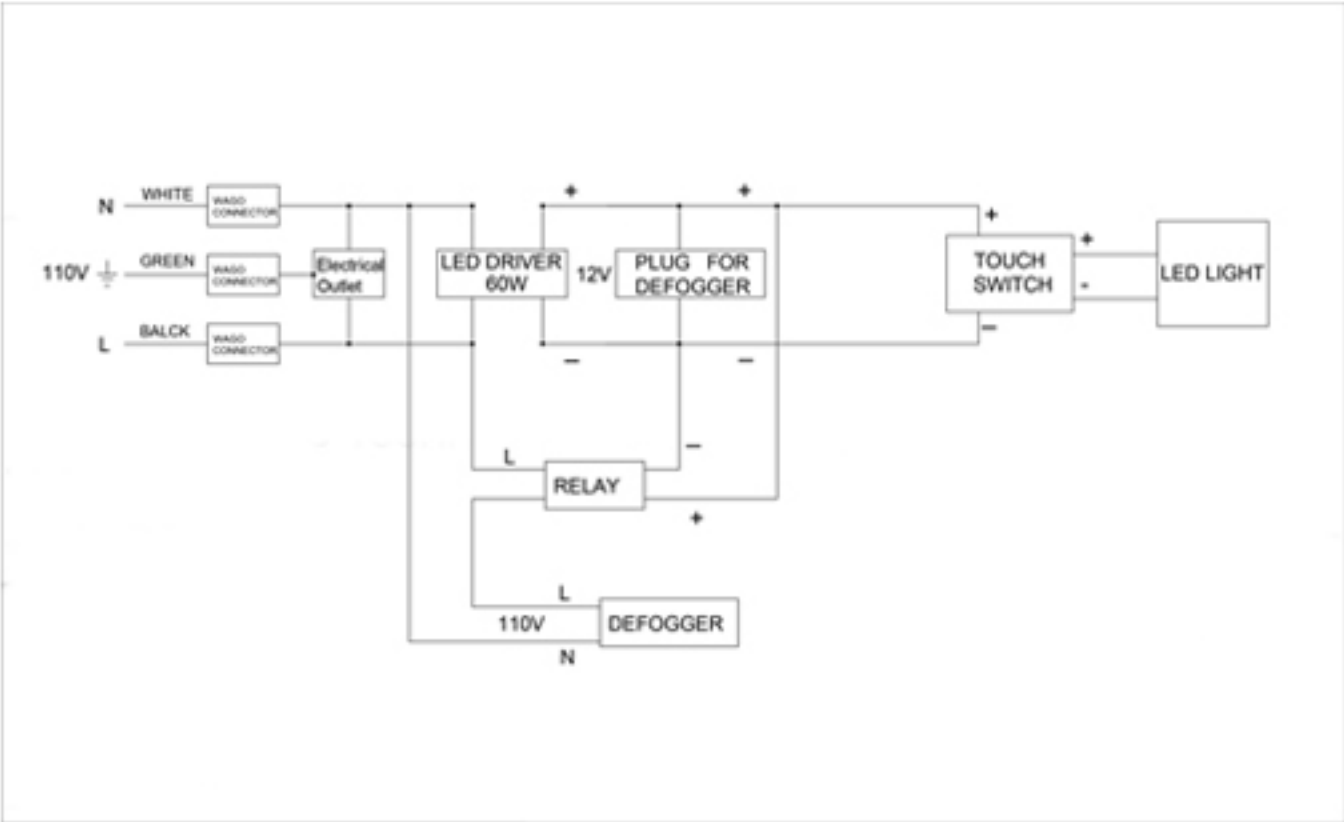
Circuit Diagram
