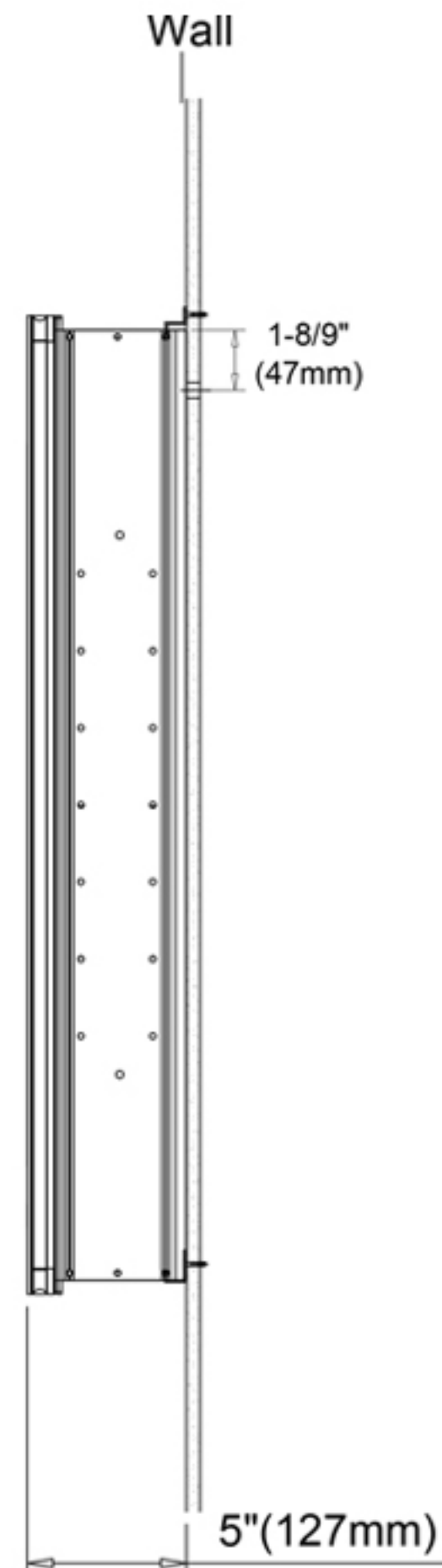
Surface Mount
