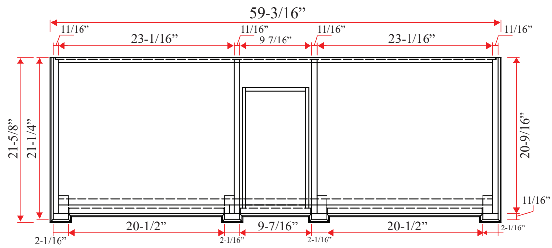
TOP VIEW
