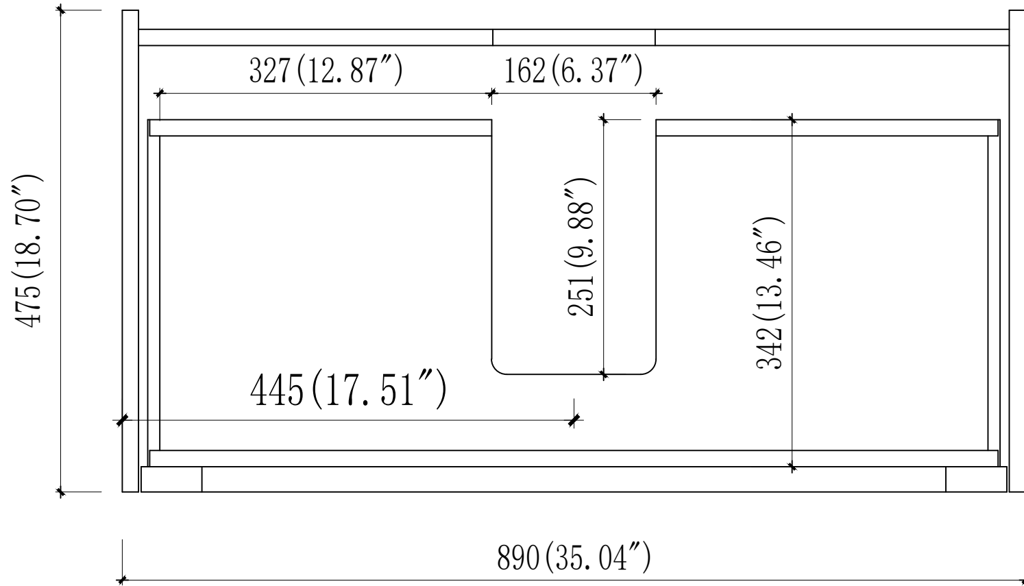
Drawer Detail
