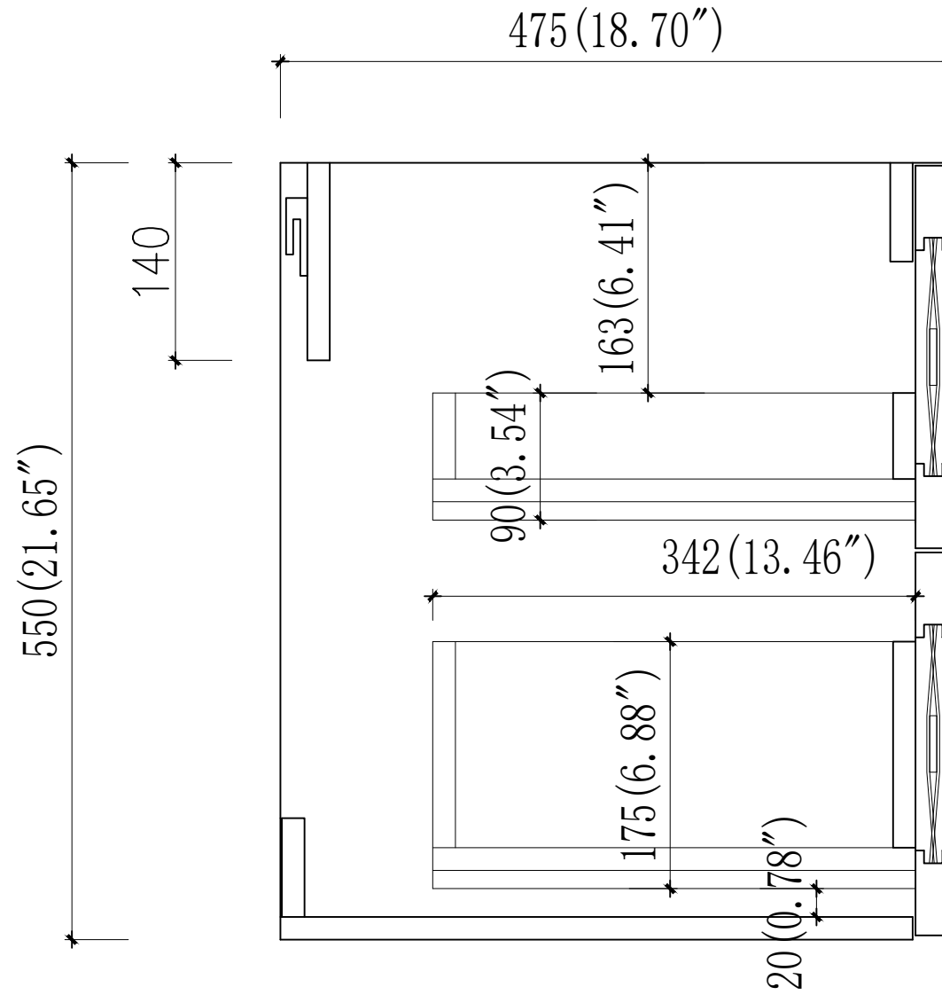
Drawer Detail
