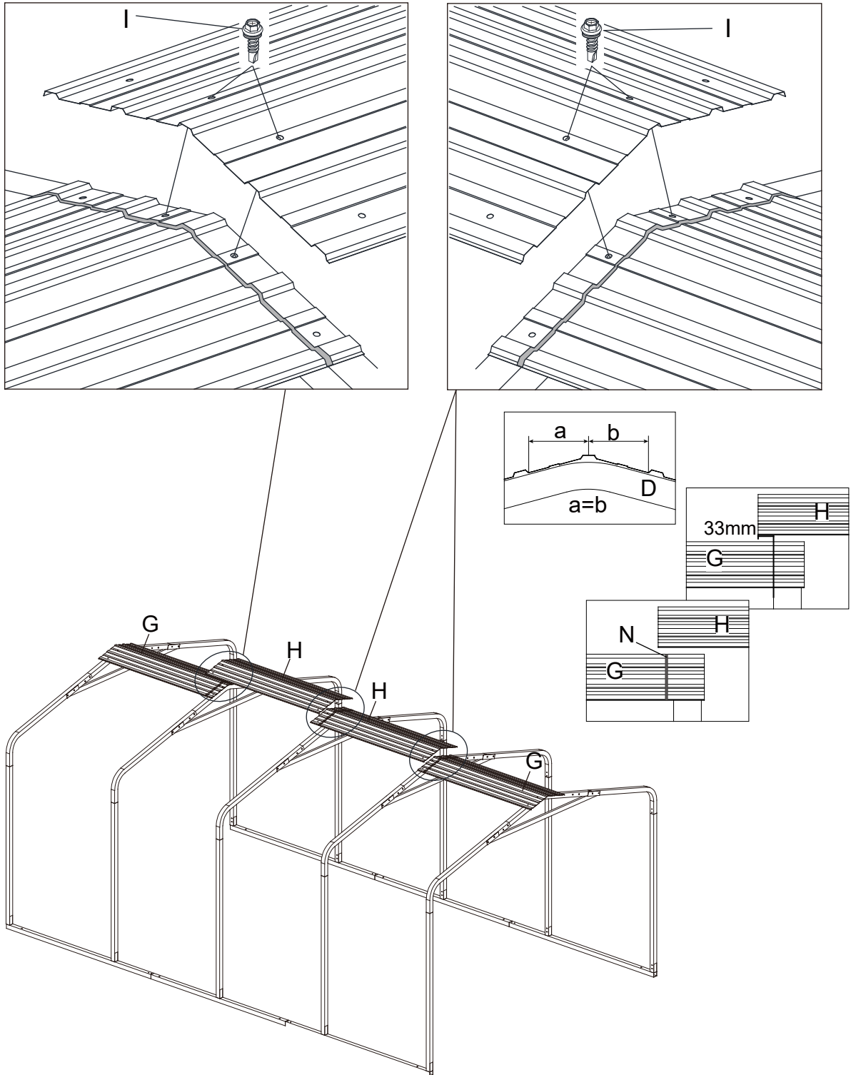
Assembly sequence for the roof sheet
