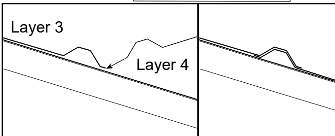
Assembly sequence for the roof sheet
