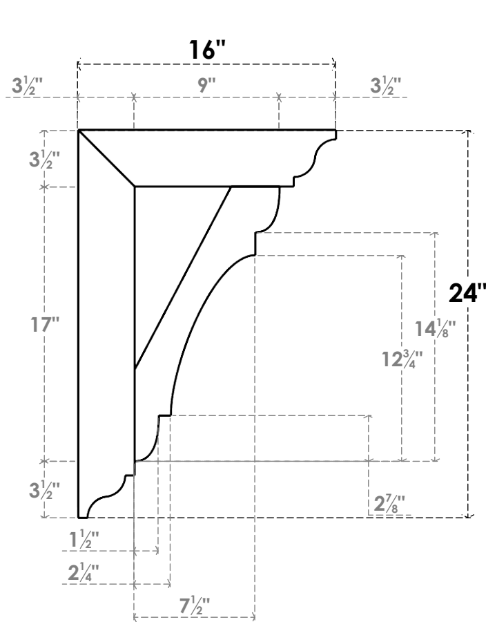
SIDE PROFILE
