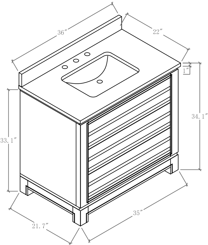
Vanity Front
