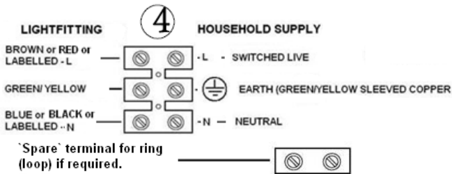
Wiring Details
