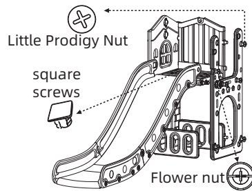
8 Attach the U-shaped side panels to the 2-lug platform and the other side of the slide
