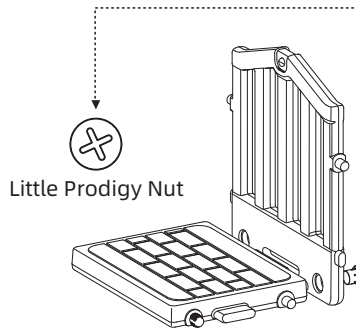
5 Platform baffle and 2-lug platform assembly
