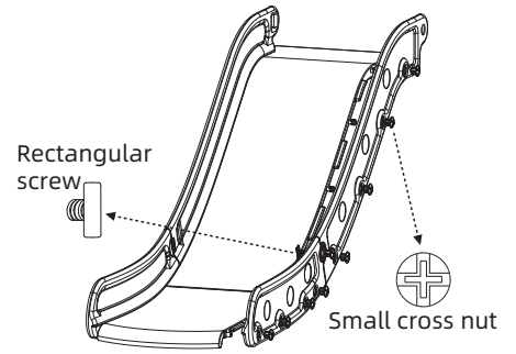
3 Fix the other side of the slide rail
