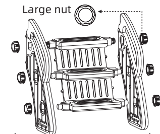
9 Use large nuts to secure the foot pedals and one-piece foot pedals to the stair railings in sequence.
