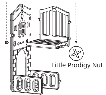
6 Secure the assembled 2-lug platform to the large side panel
