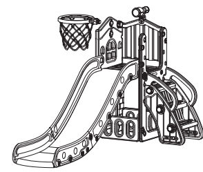
12 Use large nuts to fix the basketball hoop to the large side panel and hang the basketball net to complete the installation.
