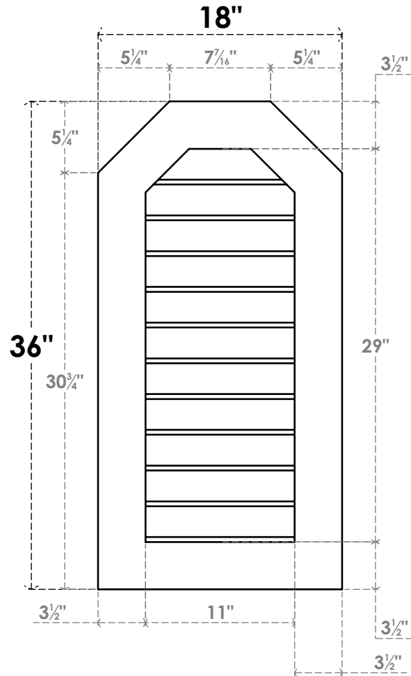
FRONT
