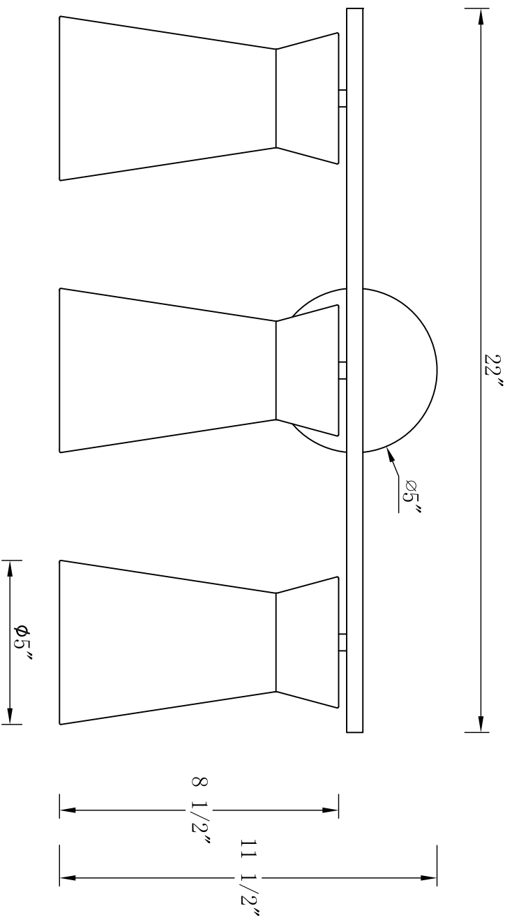
FRONT VIEW
