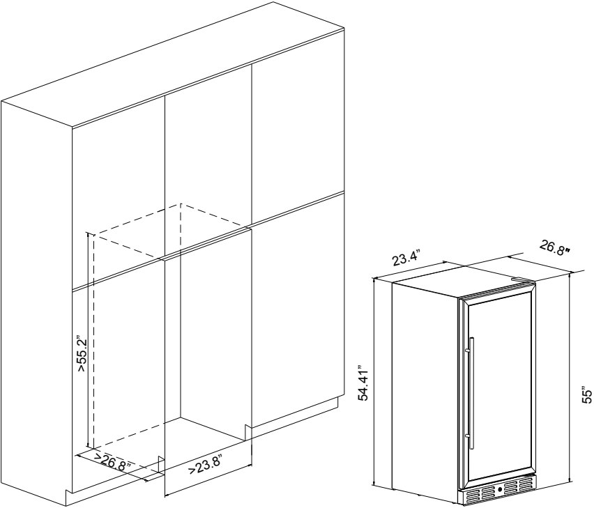
⦿ Installation Drawing
