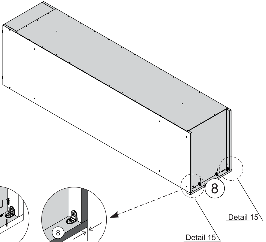
Detail 15
