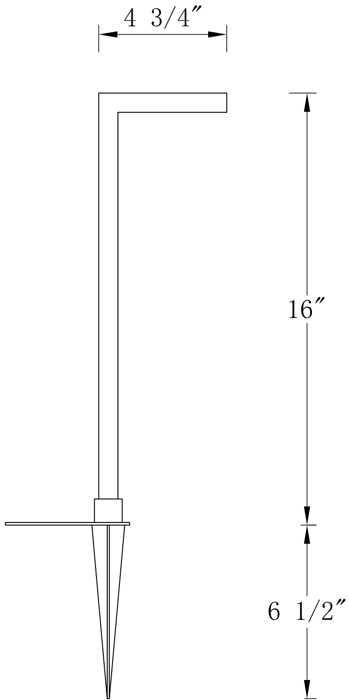
FRONT VIEW
