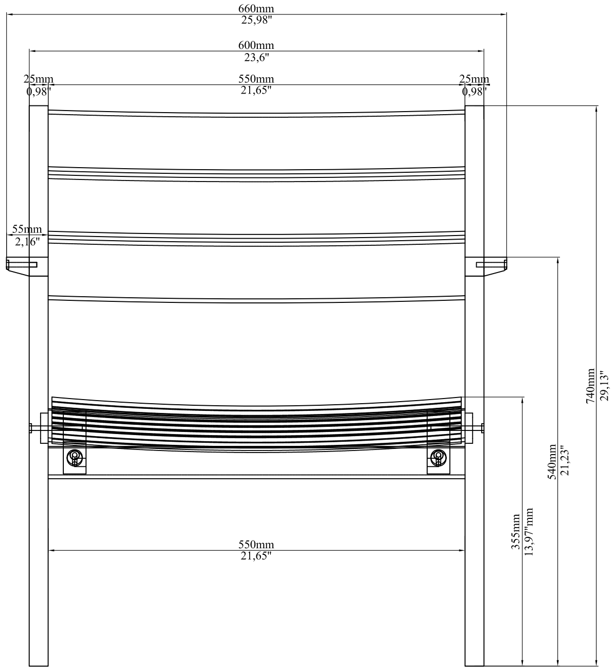
LOW CHAIR WITH BASE CUSHION
