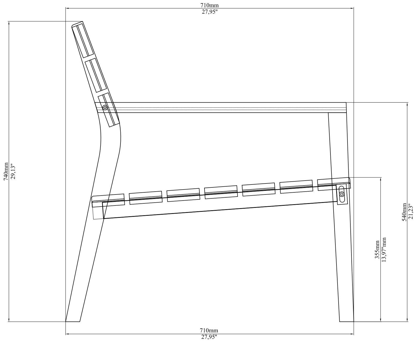
LOW CHAIR WITH BASE CUSHION
