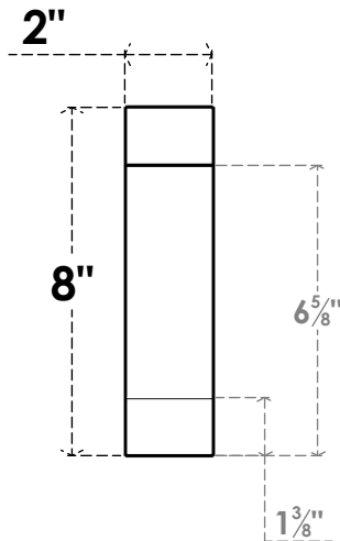
FRONT PROFILE
