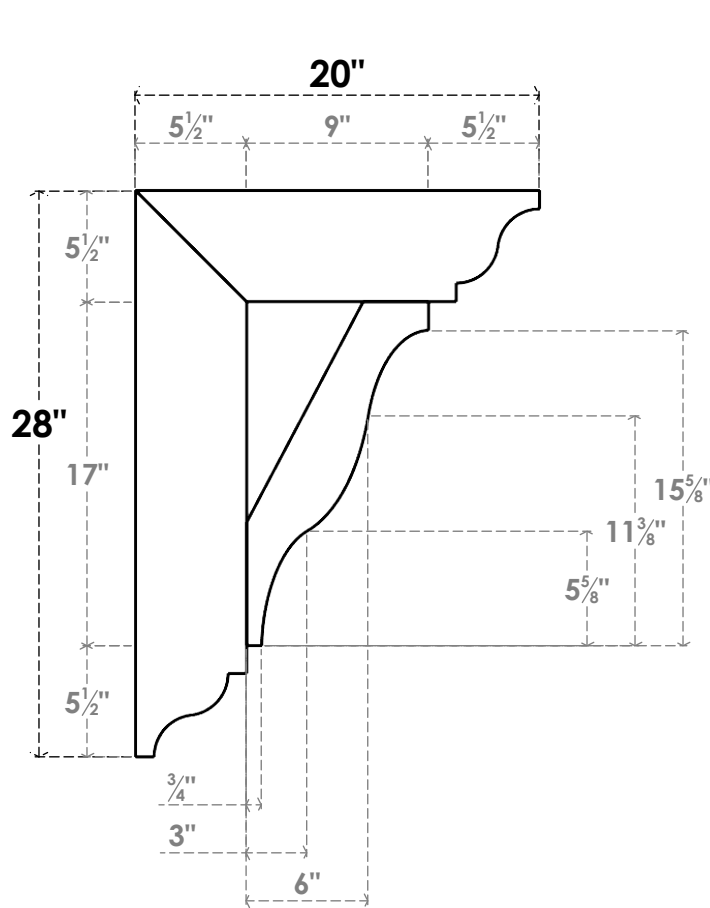
SIDE PROFILE
