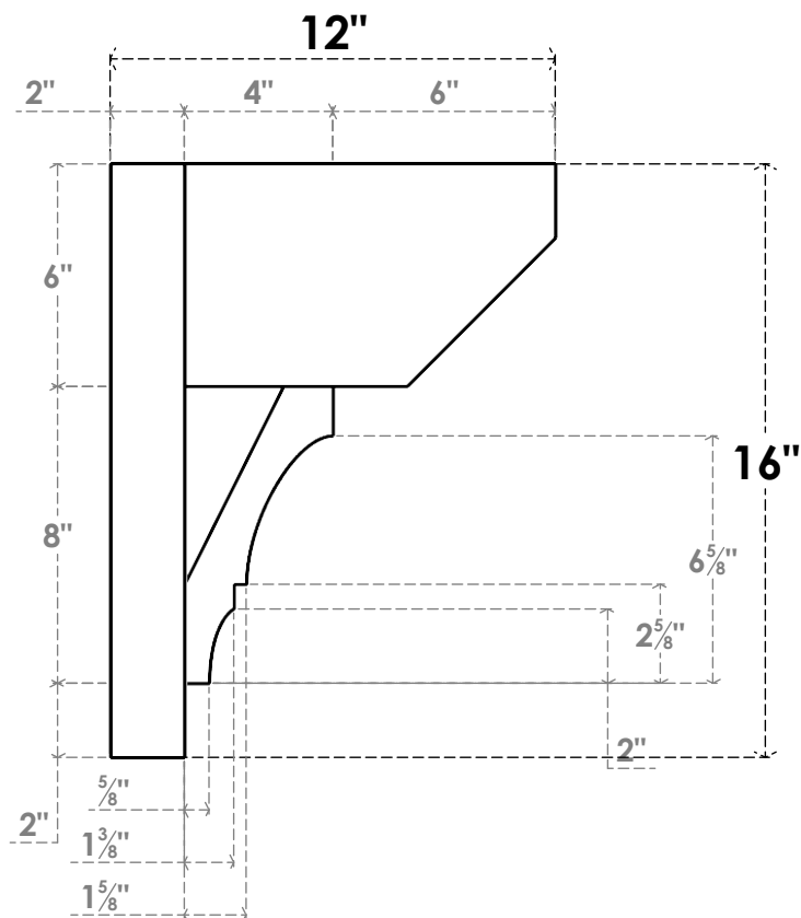
SIDE PROFILE
