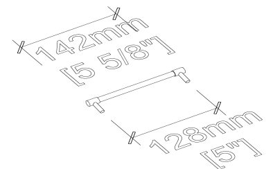
Handle's Dimension
