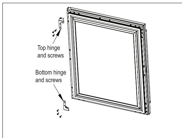
Figure 14. Door Hinges
