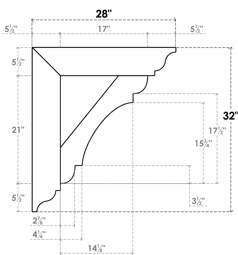
SIDE PROFILE
