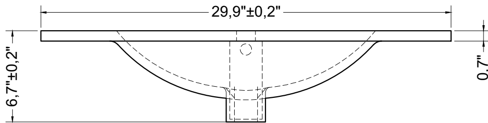
FRONT VIEW
