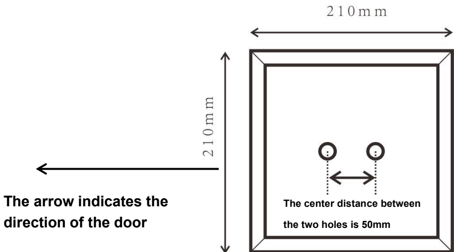
Base and mounting hole spacing dimensions
