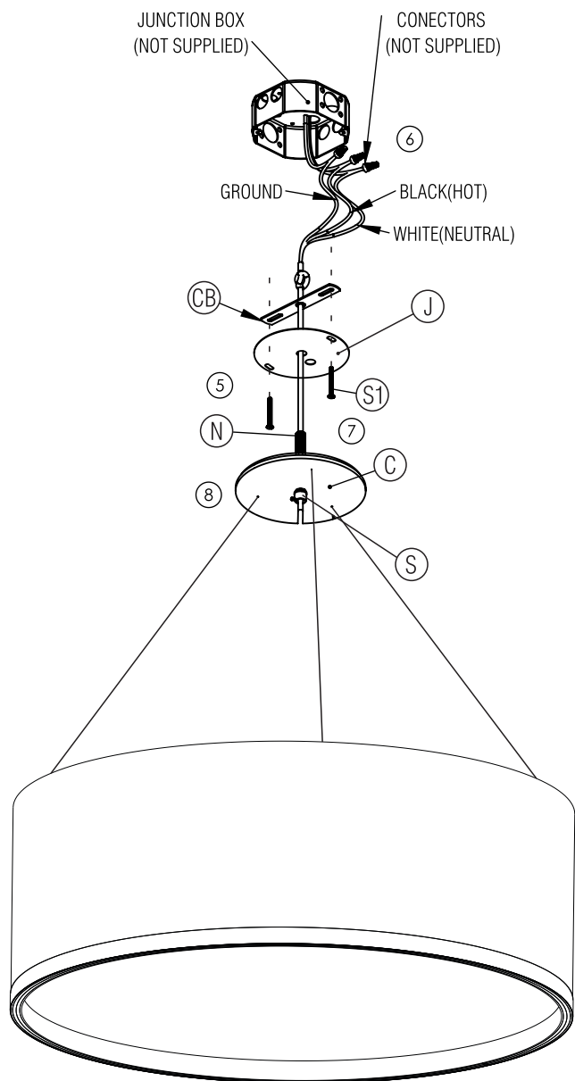
PROVIDED SCREWS
